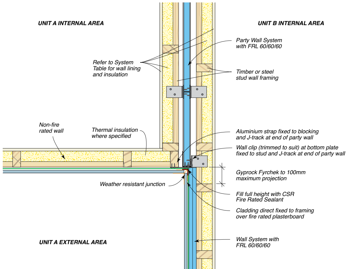
Figure 70: Junction Of Party Wall And External Wall With Cemintel Texture Base Sheet – Plan View
