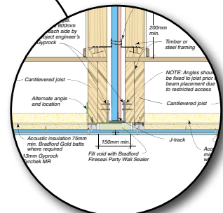
Cantilevered level soffit details. Refer to Figure 75
