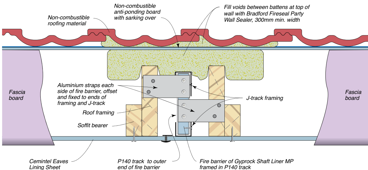
Figure 58: Eaves Detail – Outside End Elevation – Appraisal: Refer to NCC
