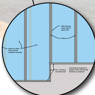
Step down details. Refer to Figure 55
