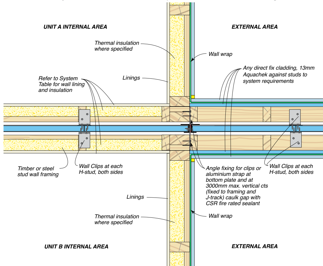
Figure 71: Junction Of Party Wall And External Wall With Aquacheck and Direct Fixed cladding – Plan View
