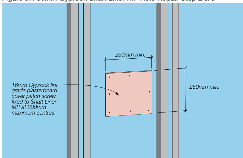
Figure 87: 50mm Gyprock Shaft Liner MP Hole Repair Step 2 & 3
