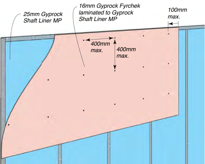
Figure 39: Installation Of Fyrchek Plasterboard Lamination (Option 1)
