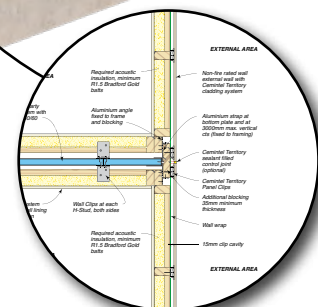
Junction of Party Wall and external walls. Refer to Figure 61
