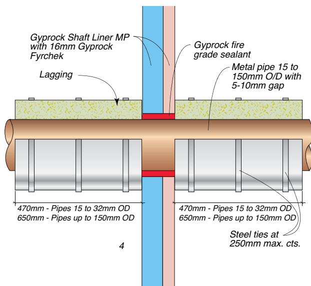
Figure 78: Metal Pipe Penetration – FRL –/90/–
