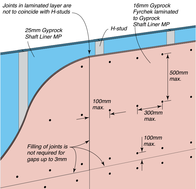
Figure 40: Installation Of Fyrchek Plasterboard Lamination (Option 2)
