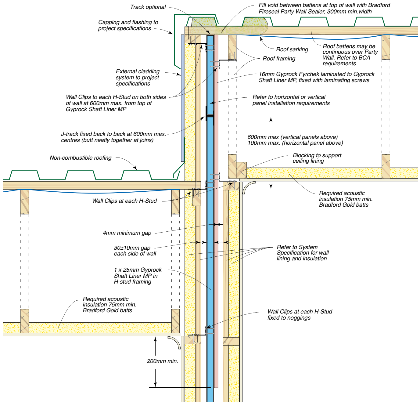
Figure 49: Detail At Stepped Roof/Ceiling
