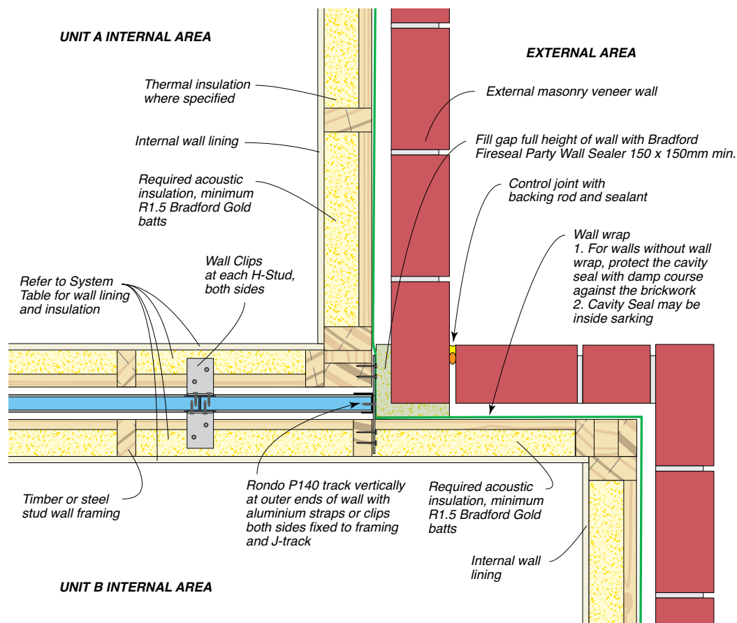
Figure 66: Junction Of Party Wall And External Wall With Brick Veneer At Wall Return – Plan View
