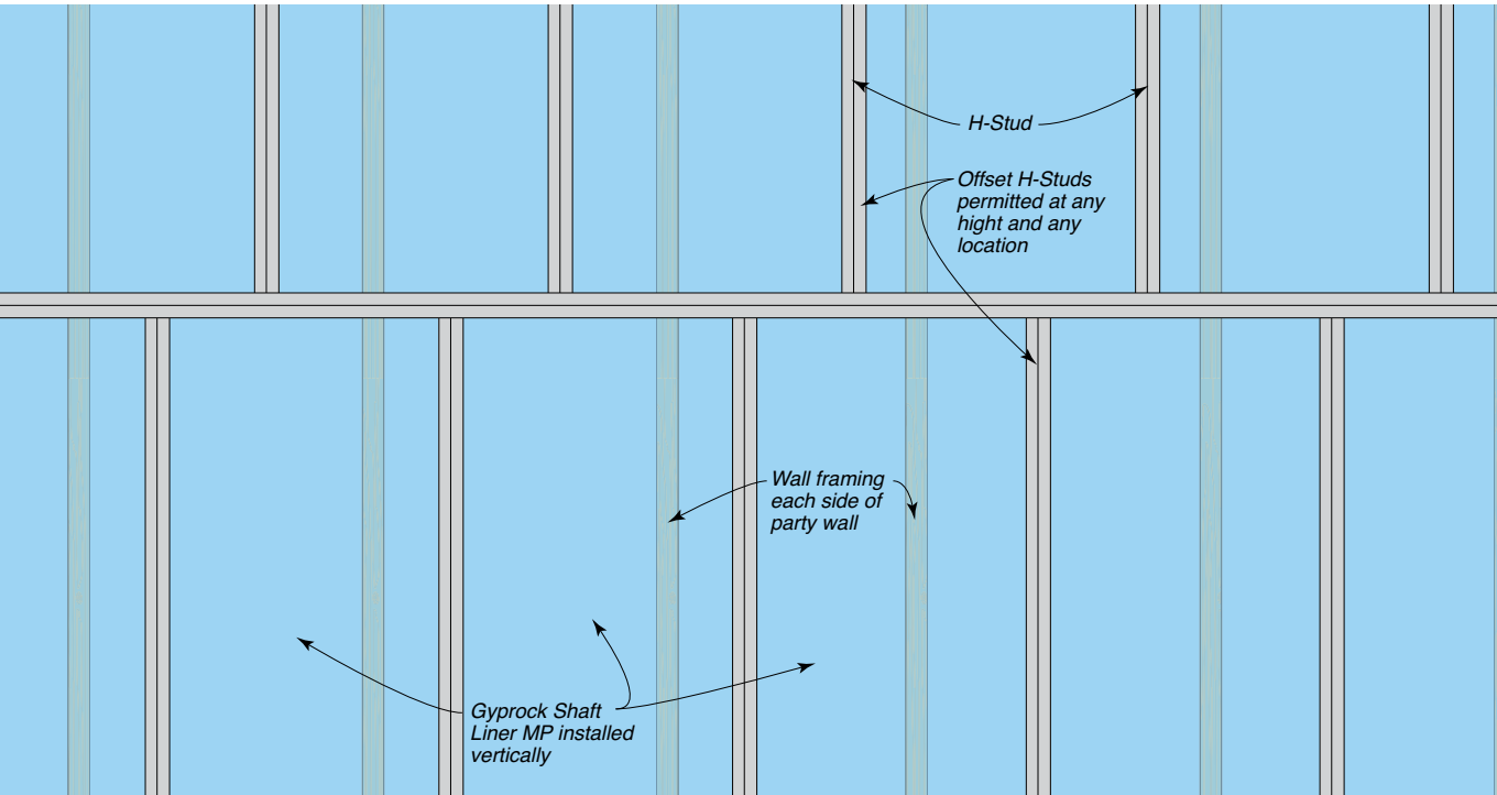
Figure 52: Offset Party Wall H-Studs (Front Elevation)
