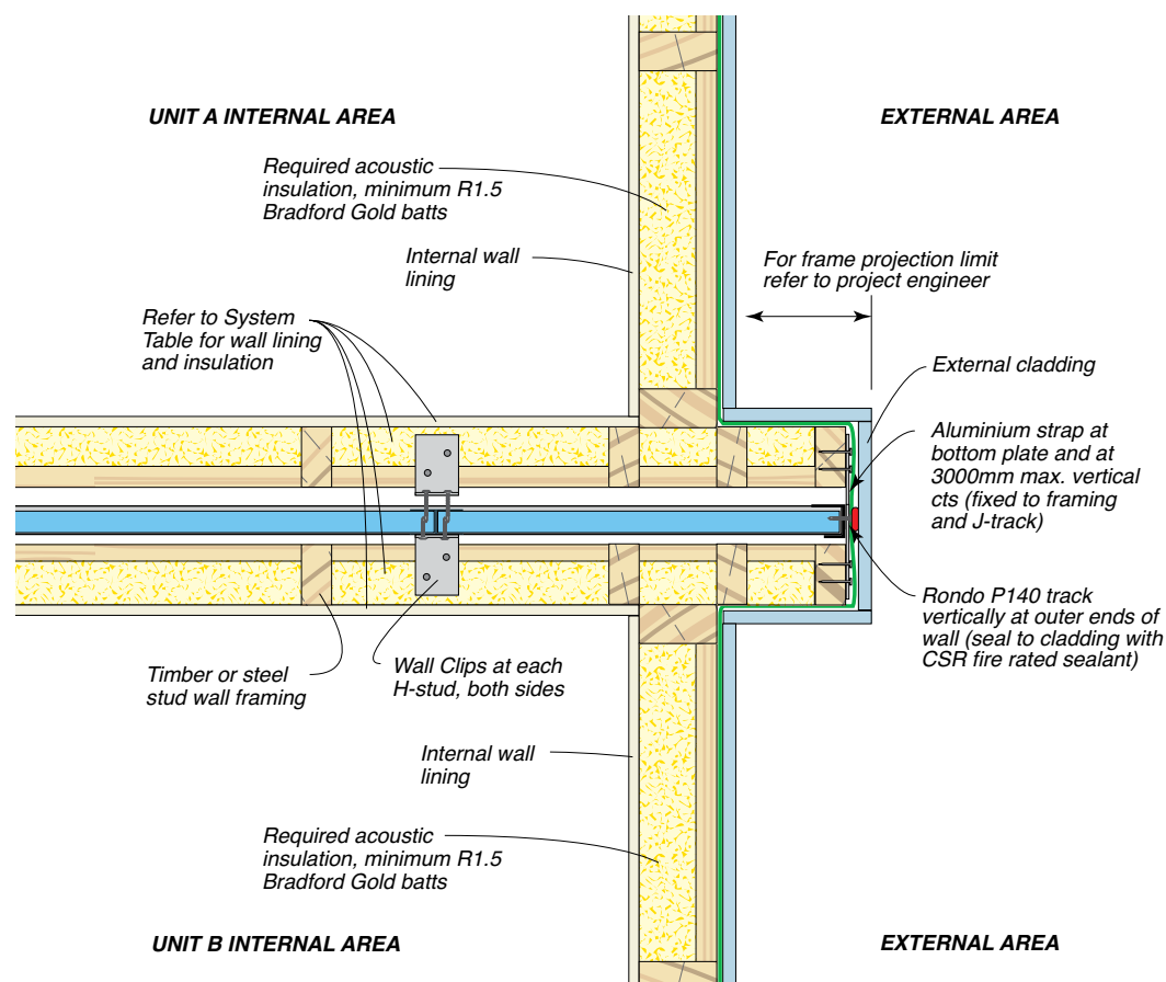
Figure 65: Junction Of Nib Party Wall And External Wall With Lightweight Cladding – Plan View
