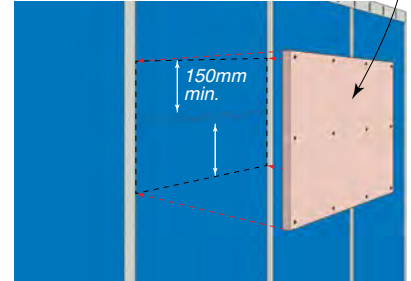
Figure 84: Gyprock Shaft Liner MP Small Crack Repair
