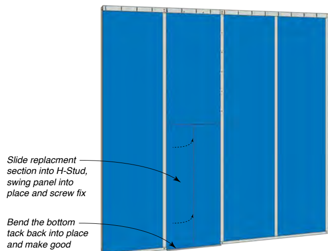
Figure 94: >300mm Gyprock Shaft Liner MP Hole Repair Step 6 & 7
