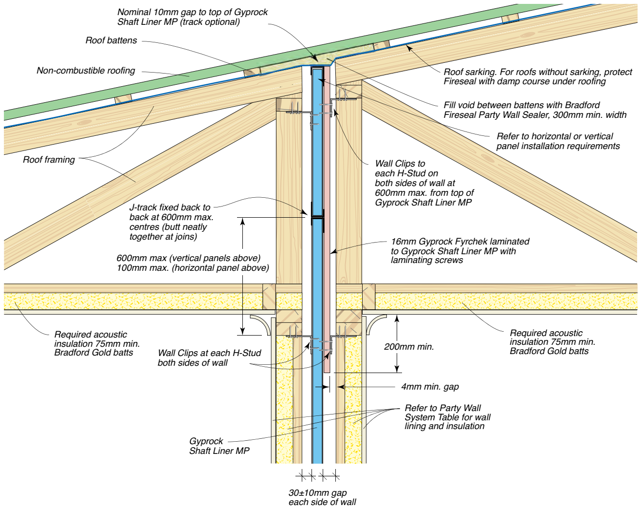
Figure 48: Detail At Roof/Ceiling With Continuous Roofing Over Party Wall
