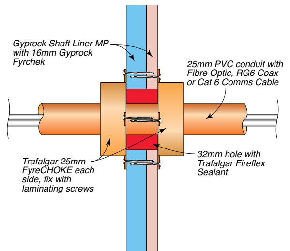
Figure 81: PVC Conduit with Communication Cable Penetration – FRL –/60/60
