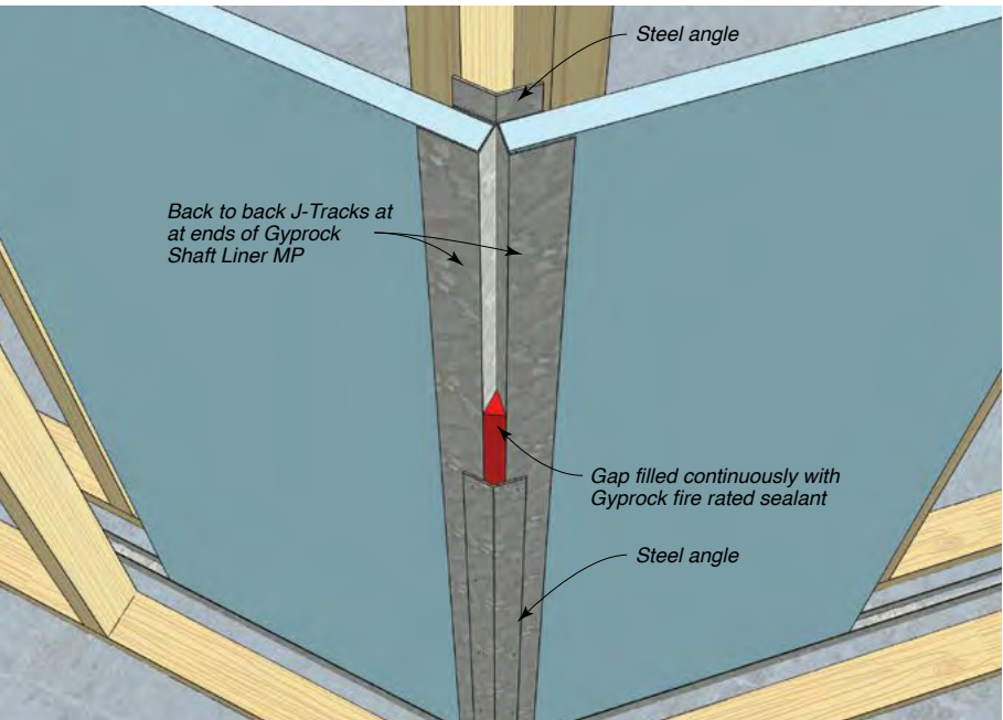
Figure 37: Party Wall 45° Corner Overview
