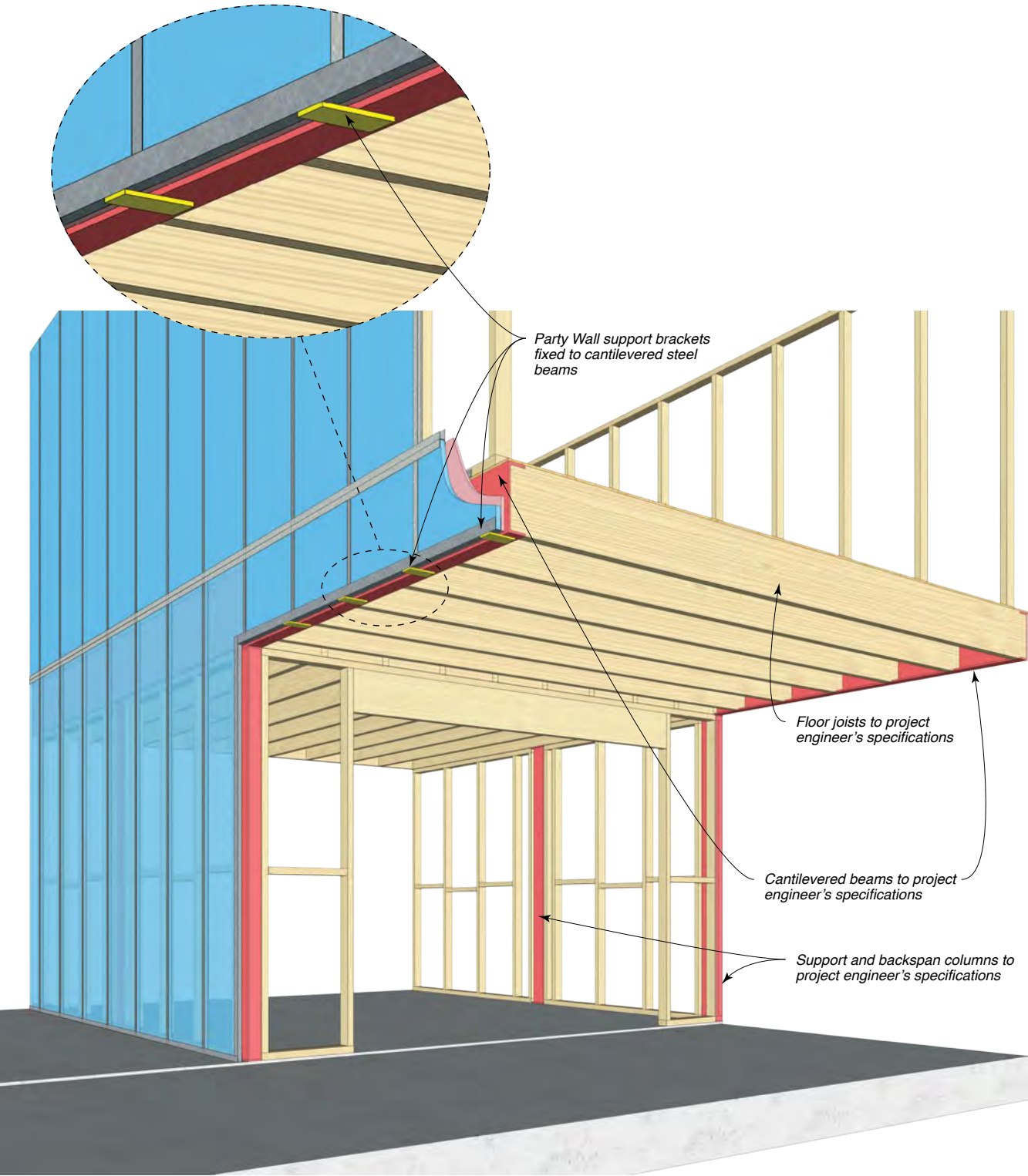
Figure 72: Cantilevered Construction Overview – Timber And Steel Framing
