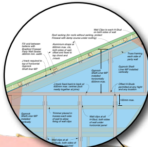
Roof and ceiling details. Refer to Figure 51
