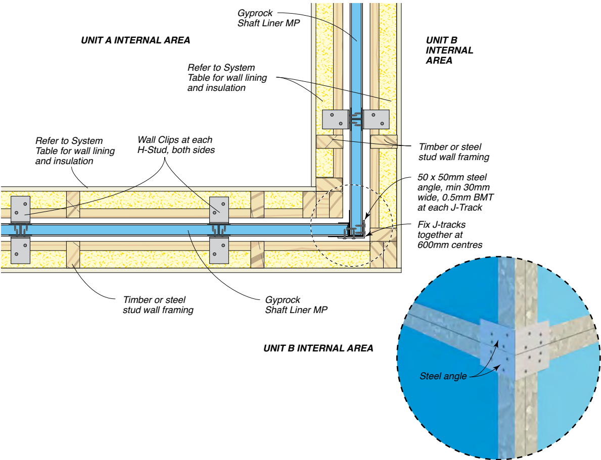
Figure 31: Junction Of Party Wall And Party Wall At Corner (clip on internal side)– Plan View
