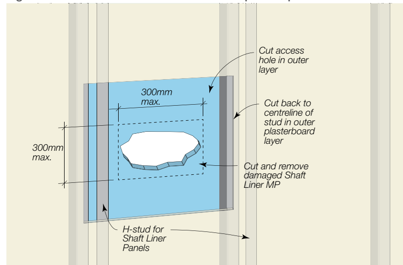
Figure 89: <300mm Shaft Liner MP Hole Repair Step 1 & 2
