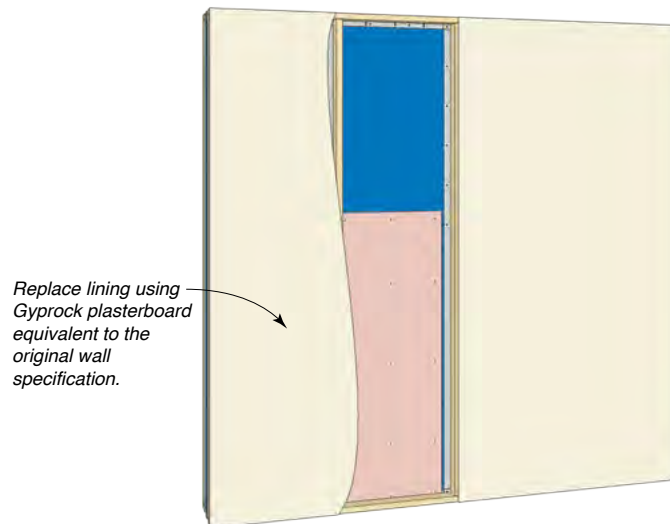
Figure 96: >300mm Gyprock Shaft Liner MP Hole Repair Step 9
