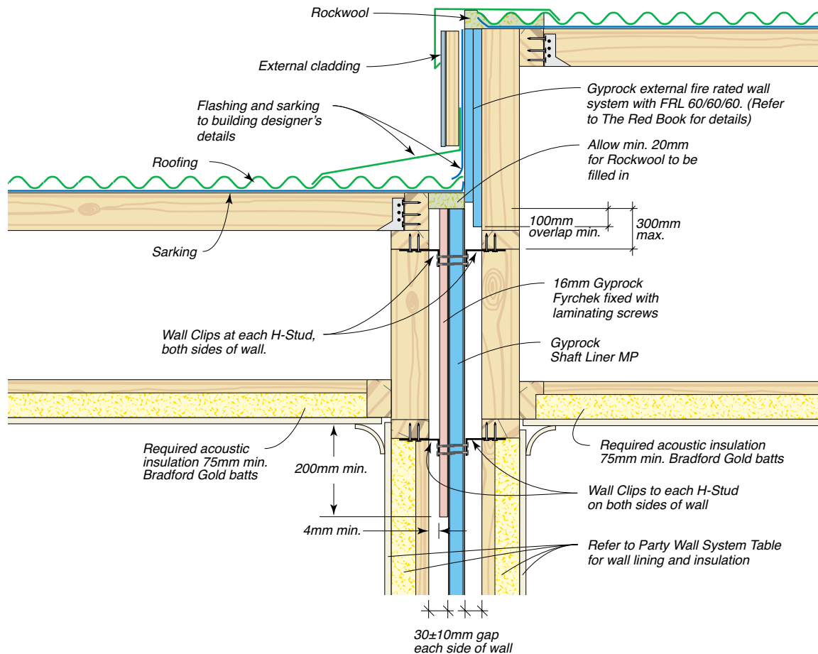
Figure 44: Detail At Roof/Ceiling At Transition From Single To Two Storey
