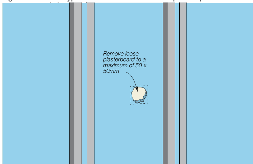
Figure 86: 50mm Gyprock Shaft Liner MP Hole Repair Step 1
