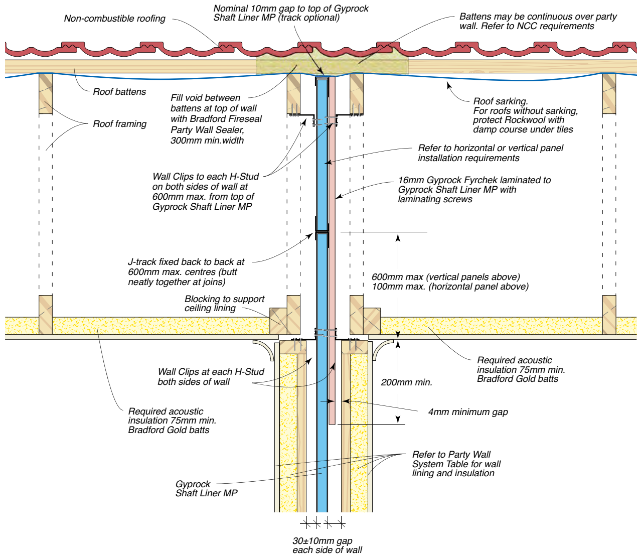
Figure 45: Detail At Ceiling And Roof
