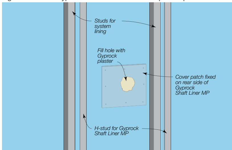
Figure 88: 50mm Gyprock Shaft Liner MP Hole Repair Step 4
