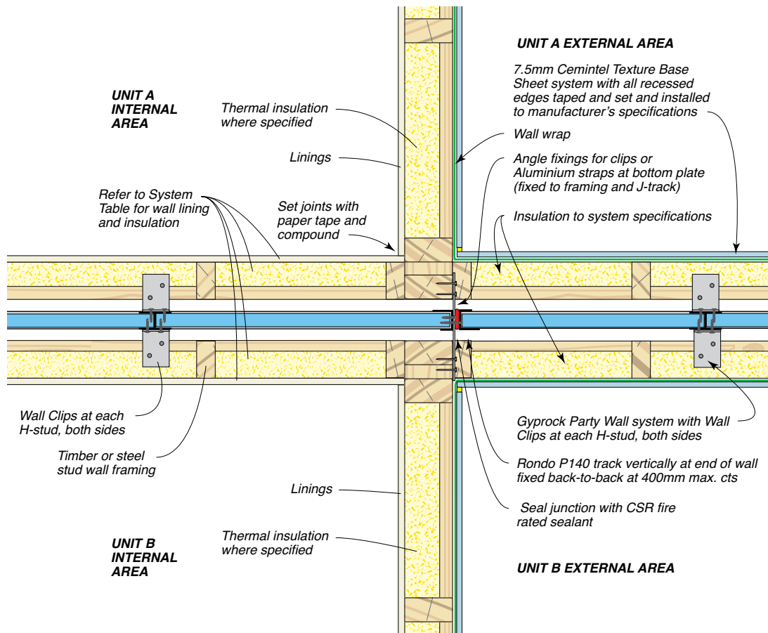
Figure 70: Junction Of Party Wall And External Wall With Cemintel Texture Base Sheet – Plan View
