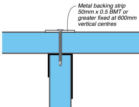
Figure 34: Fixing Method 1
