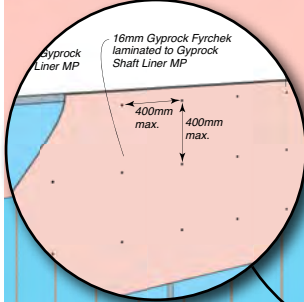
Party Wall Junction details. Refer to Figure 39 & Figure 40
