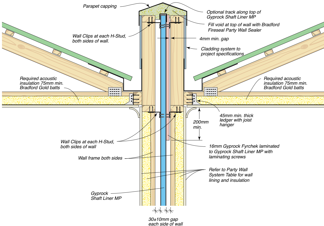
Figure 47: Detail At Roof/Ceiling And Parapet
