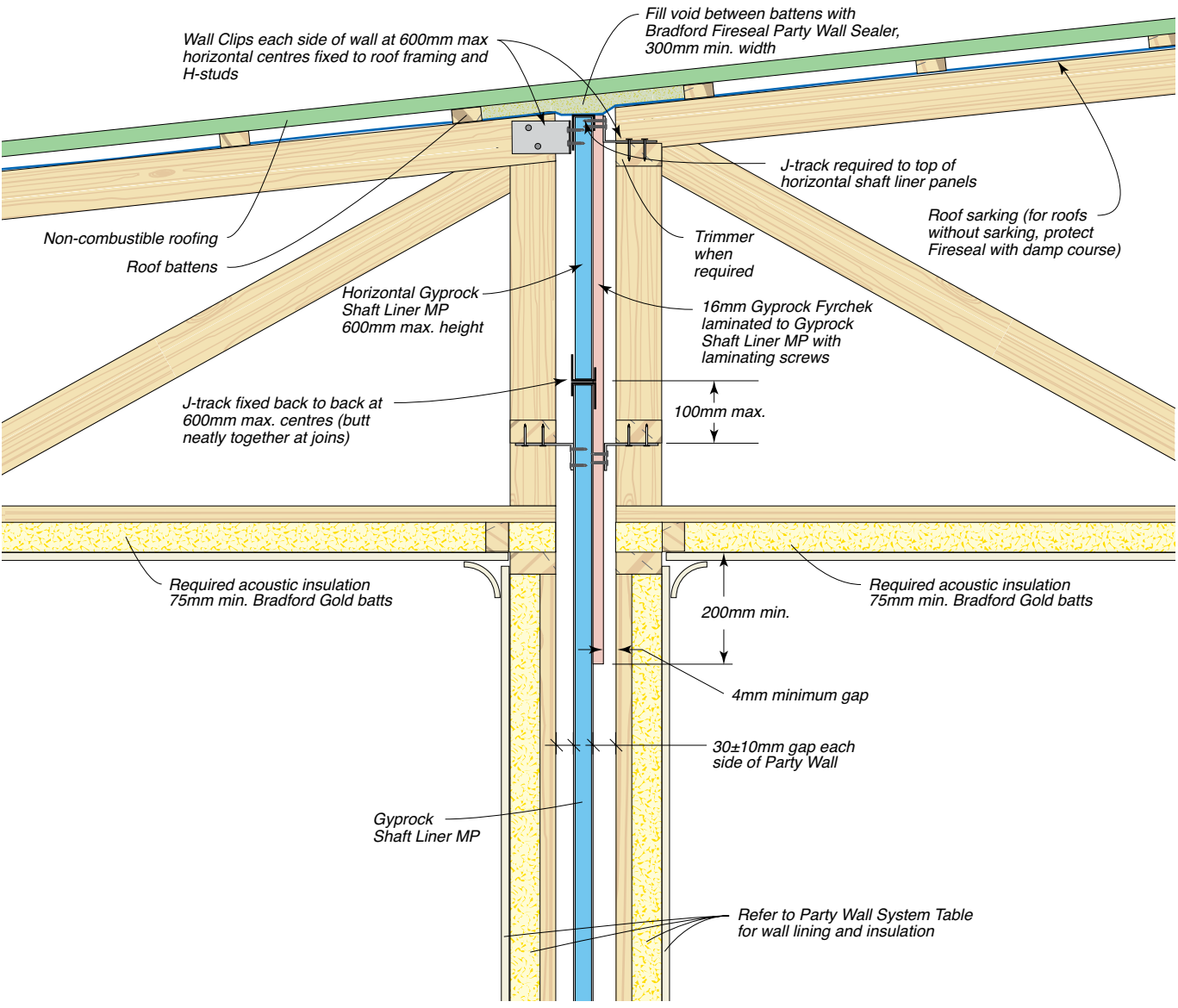
Figure 56: Roof Void With Horizontal Over Vertical Panels – Party Wall Perpendicular to Truss/Rafter ( Side Elevation)
