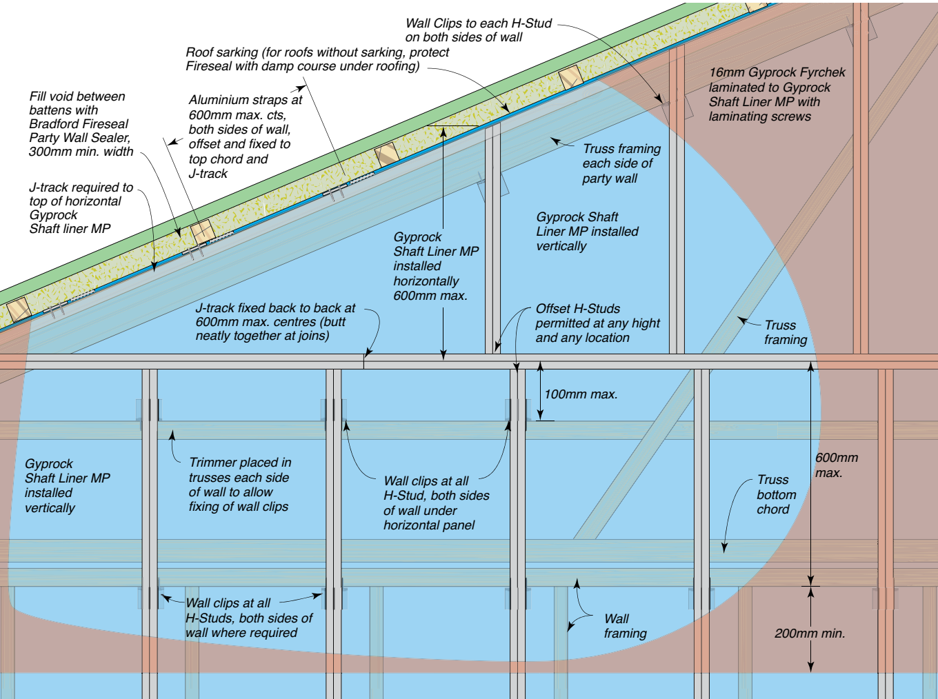
Figure 52: Offset Party Wall H-Studs (Front Elevation)
