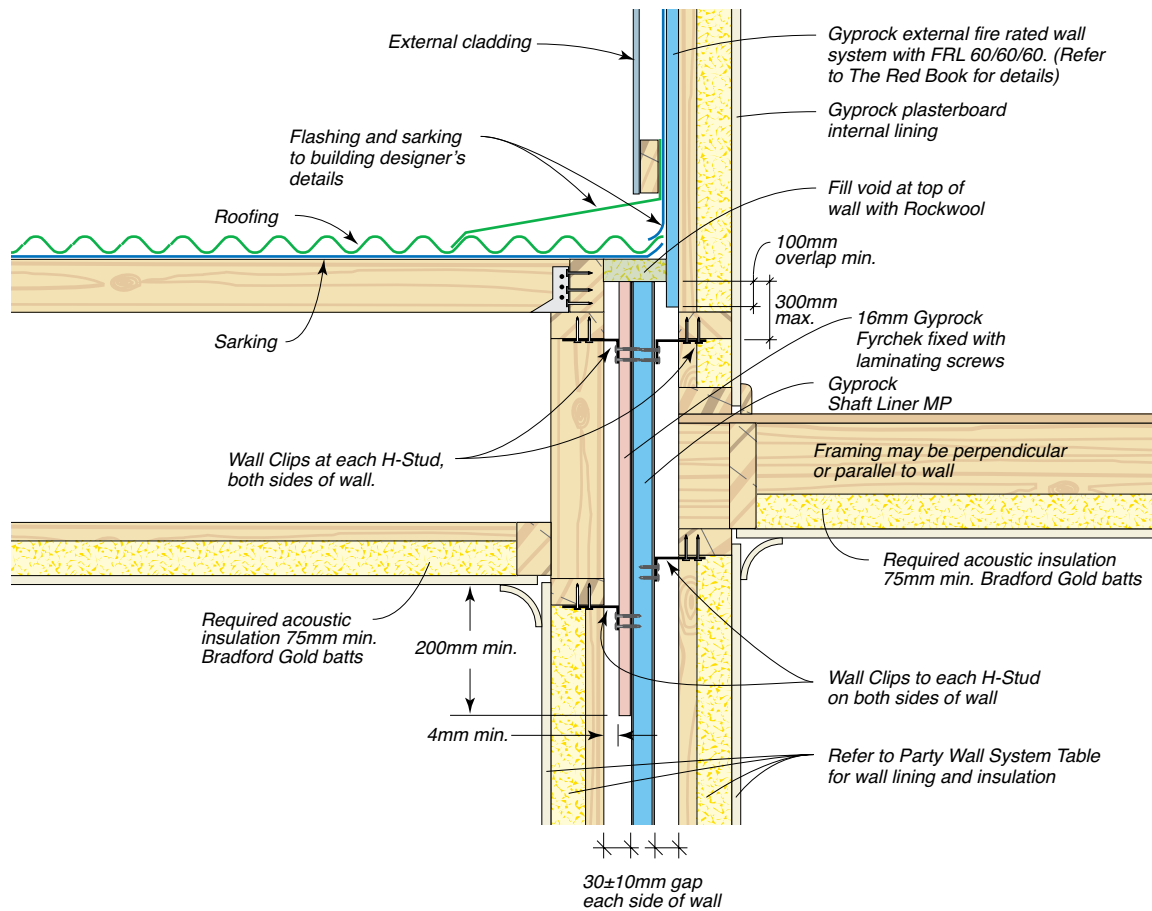
Figure 44: Detail At Roof/Ceiling At Transition From Single To Two Storey
