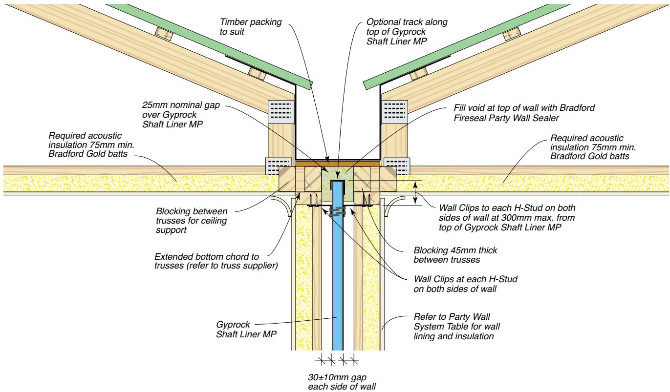
Figure 46: Detail At Roof/Ceiling And Valley Gutter
