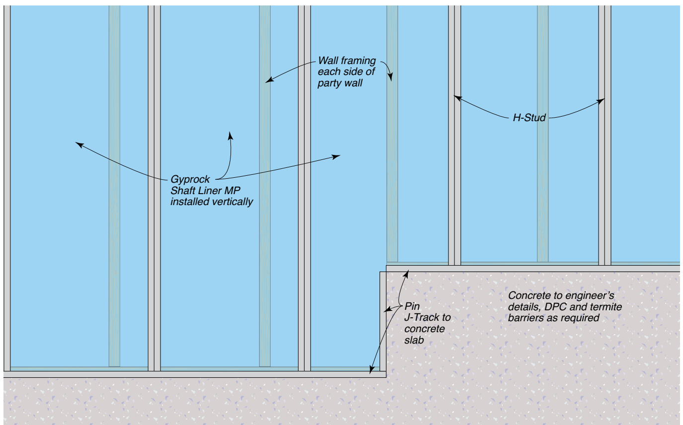
Figure 55: Floor Step Down with Vertical Shaft Liner MP – (Front Elevation)
