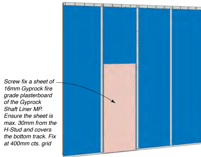
Figure 95: >300mm Gyprock Shaft Liner MP Hole Repair Step 8
