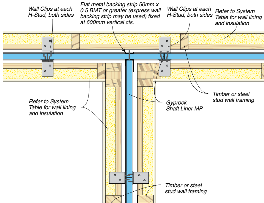
Figure 34: Fixing Method 1
