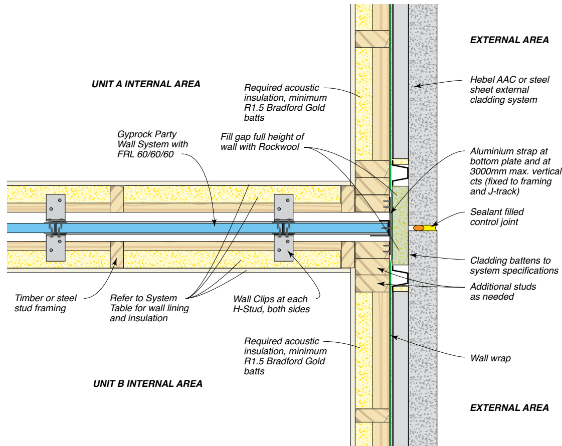
Figure 62: Junction Of Party Wall And External Wall With Hebel AAC Or Steel Sheet Cladding – Plan View
