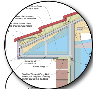
Eaves details. Refer to Figure 57
