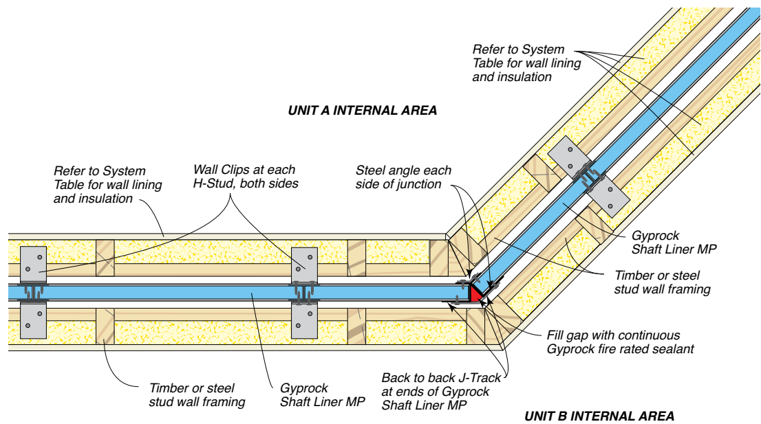
Figure 36: Party Wall 45° Corner – Plan View
