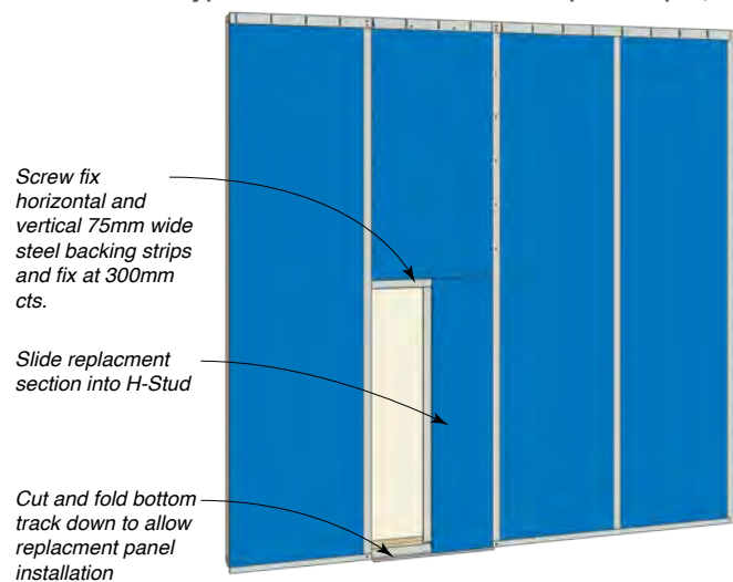
Figure 93: >300mm Gyprock Shaft Liner MP Hole Repair Step 3, 4 & 5
