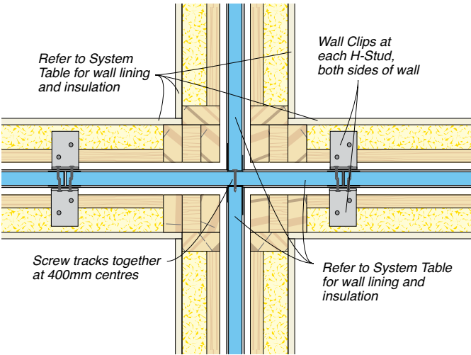
Figure 38: Junction Party Wall To Party Wall At 4-Way Intersection – Plan View
