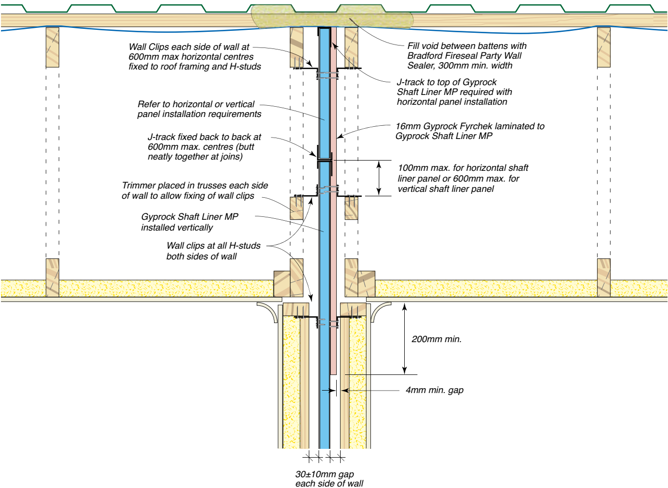
Figure 53: Roof Void With Horizontal & Vertical Panels – Party Wall Parallel to Truss/Rafter (Side Elevation)
