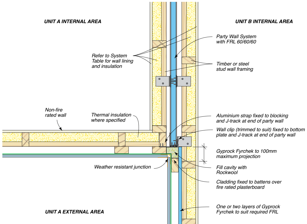
Figure 68: Junction Of Party Wall And External Wall With Lightweight Cladding At Wall Return – Cavity System – Plan View
