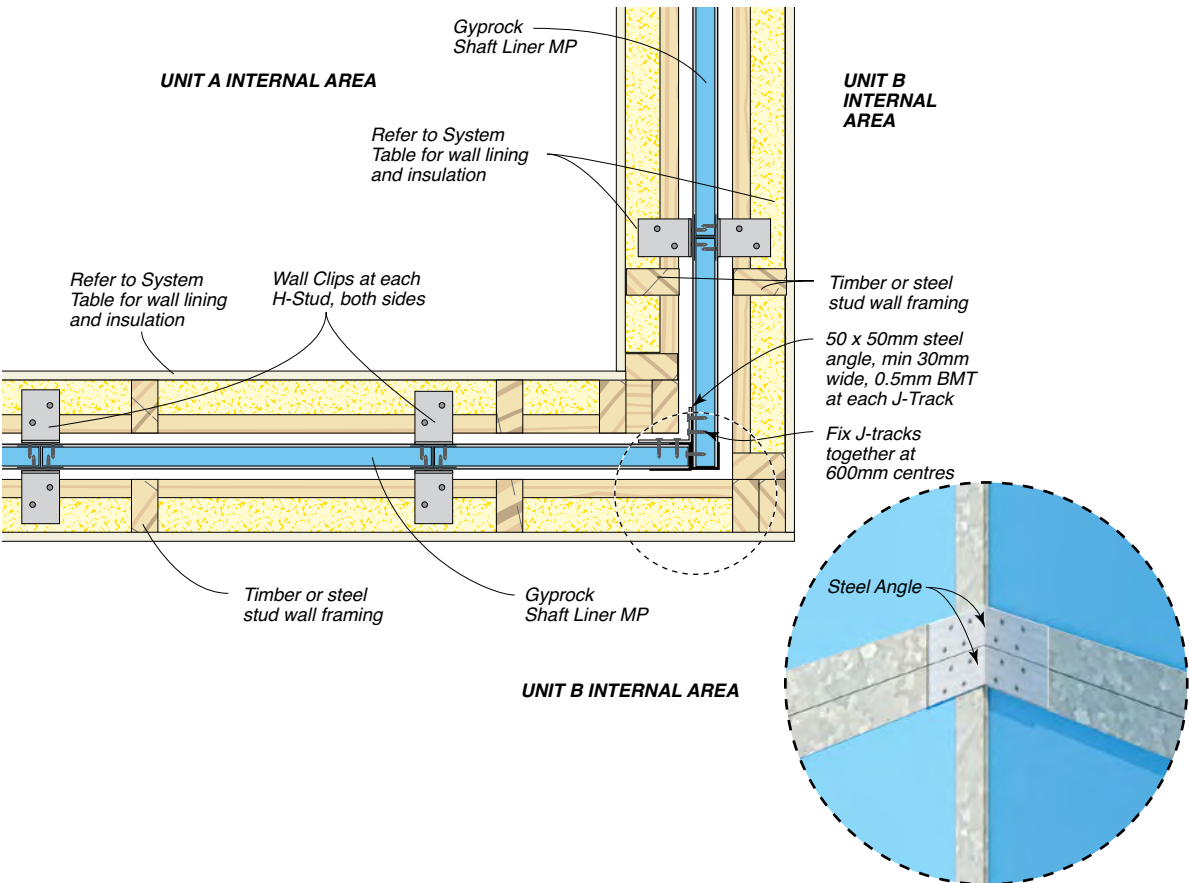
Figure 31: Junction Of Party Wall And Party Wall At Corner (clip on internal side)– Plan View
