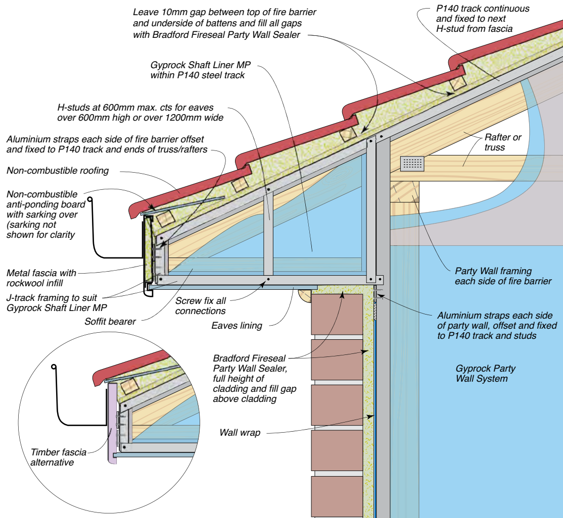
Figure 57: Eaves Detail Fascia – Front Elevation – Appraisal: Refer to BCA
