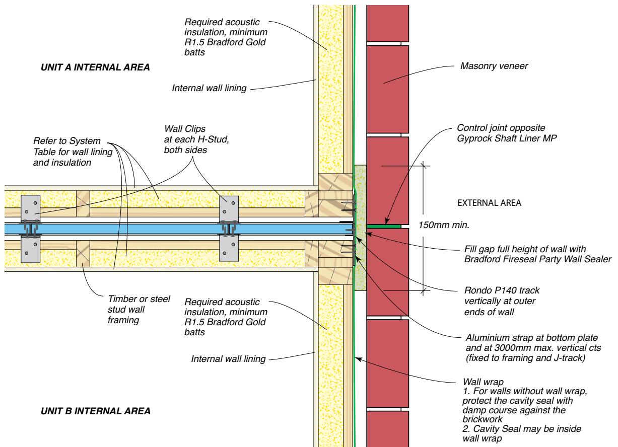
Figure 64: Junction Of Party Wall And External Brick Veneer Wall – Plan View
