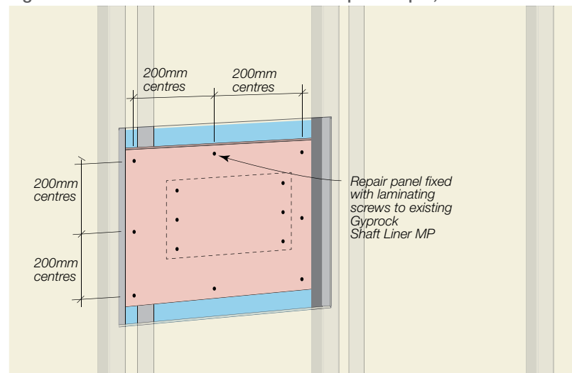
Figure 91: <300mm Shaft Liner MP Hole Repair Step 5,6 &7
