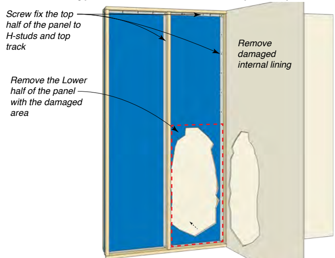
Figure 92: >300mm Gyprock Shaft Liner MP Hole Repair Step 1 & 2
