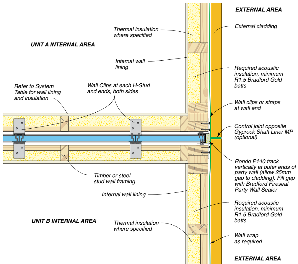
Figure 60: Junction Of Party Wall And External Wall With Lightweight Cladding Direct Fixed to Studs – Plan View
