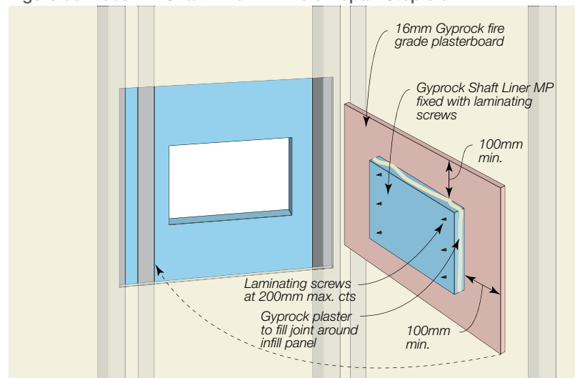
Figure 90: <300mm Shaft Liner MP Hole Repair Step 3 & 4
