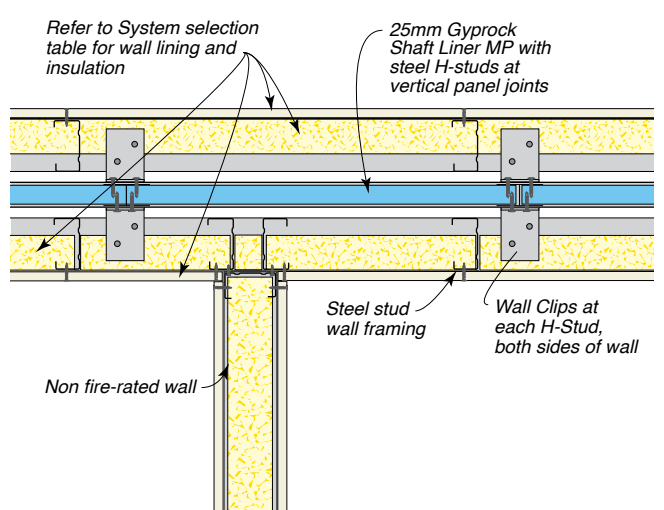
Figure 29: Junction Of Party Wall And Non-Fire Rated Internal Steel Frame Wall (Option 3) - Plan View
