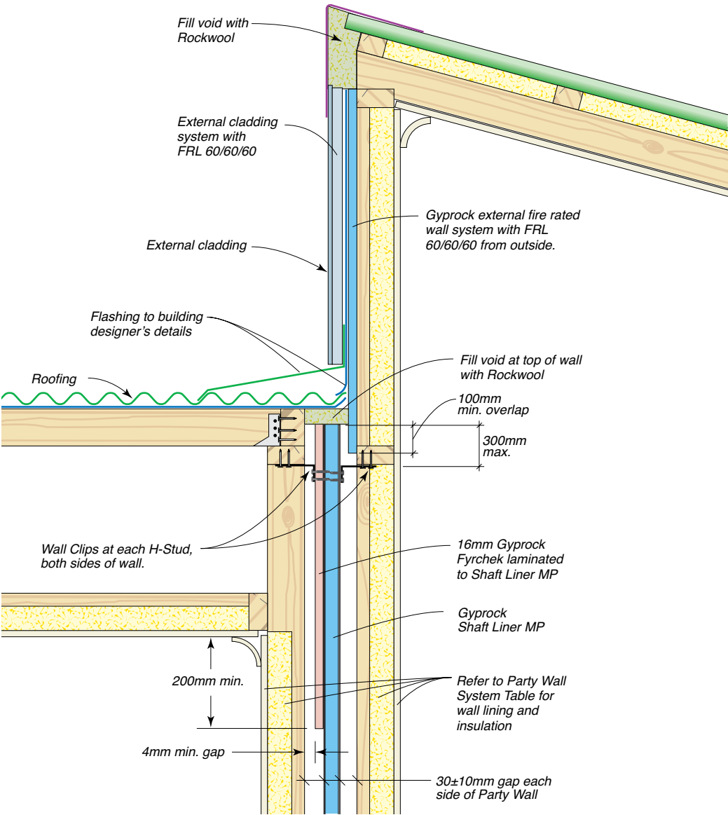
Figure 50: Roof With Party Wall To Underside Of Lower Roof Line
