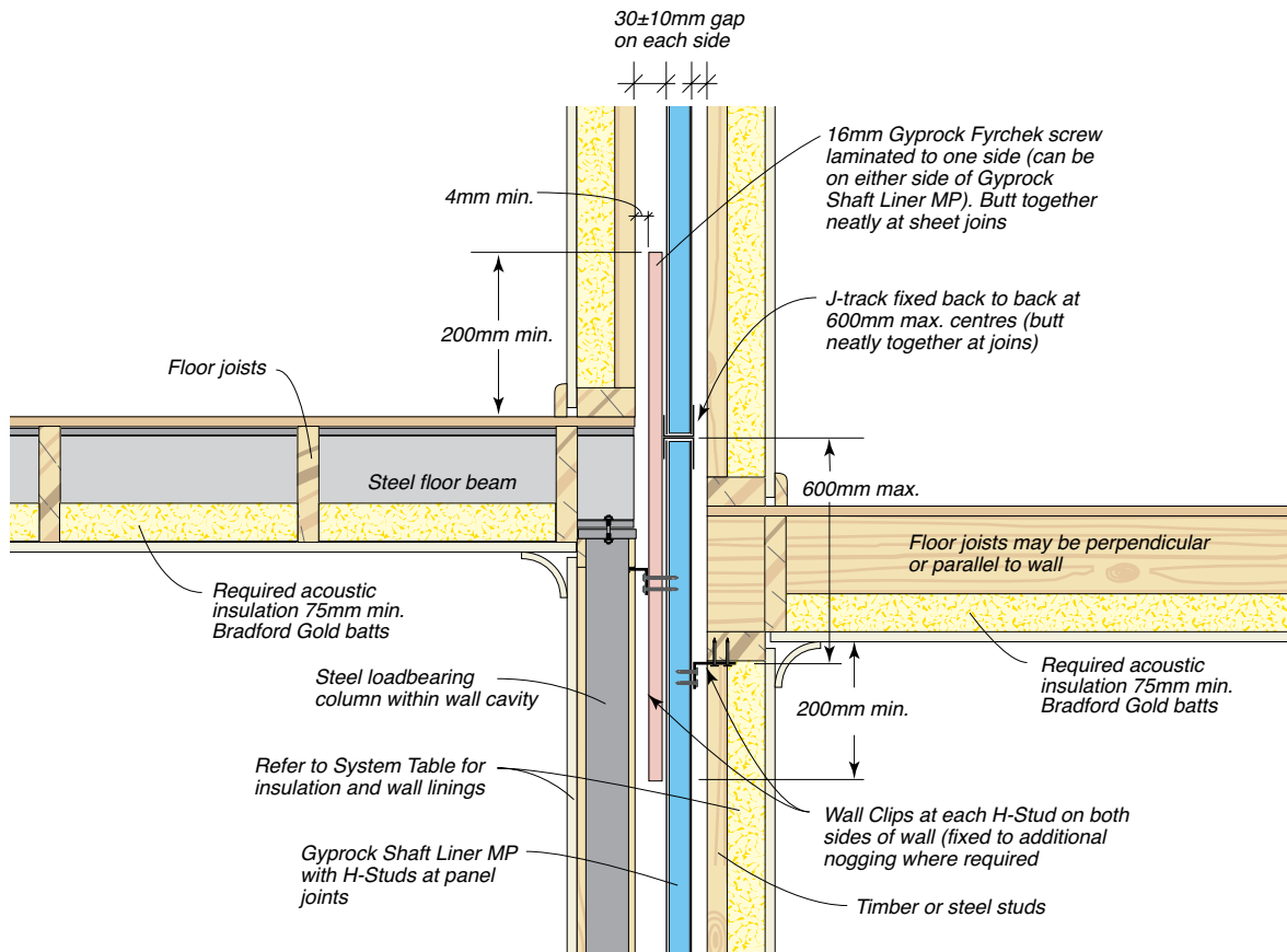
Figure 42: Detail For Steel Column And Beam Support
