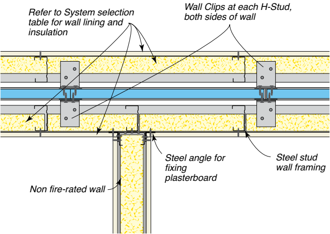
Figure 29: Junction Of Party Wall And Non-Fire Rated Internal Steel Frame Wall (Option 3) - Plan View
