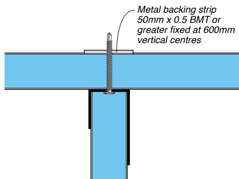
Figure 35: Fixing Method 2
