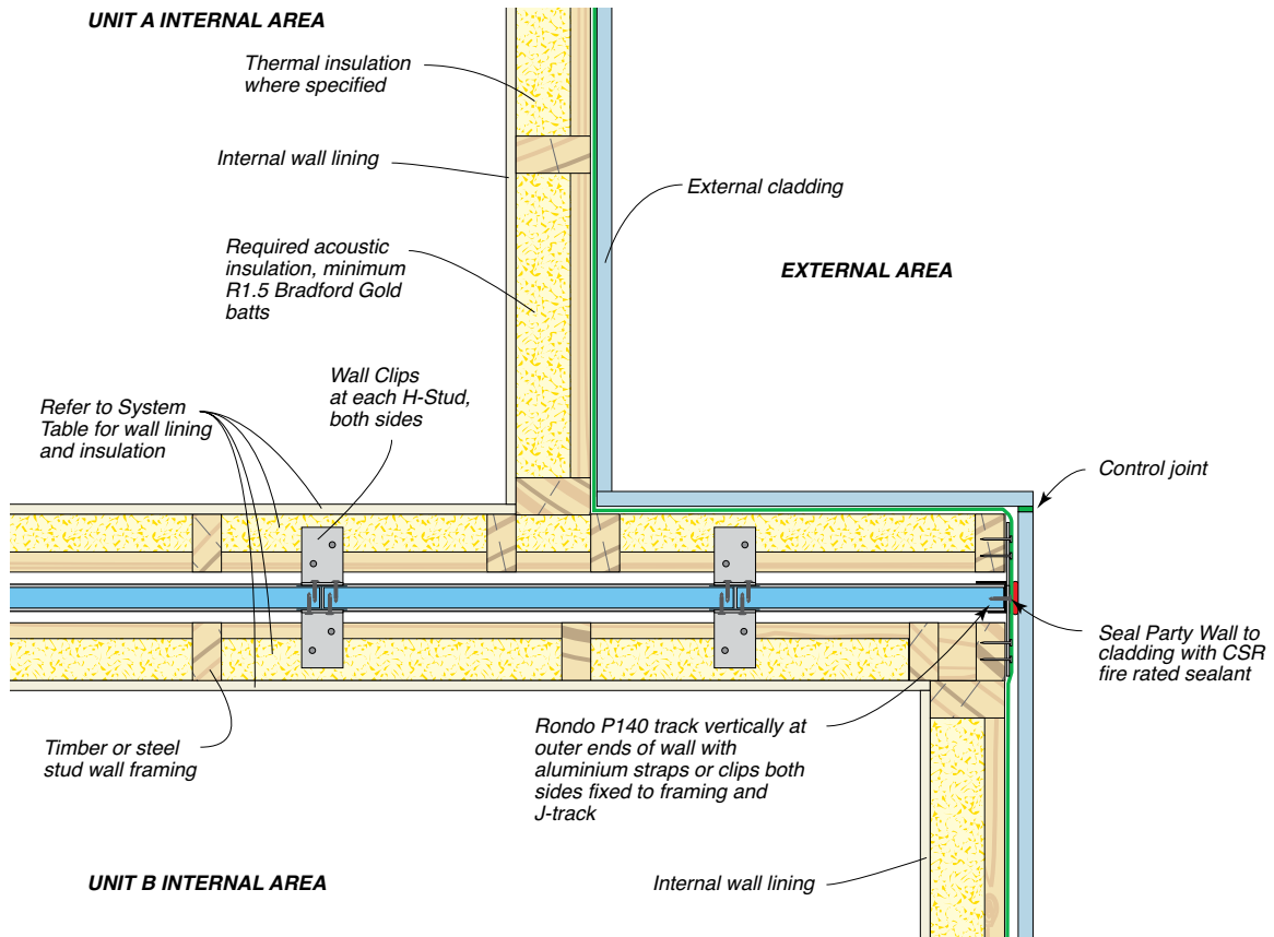
Figure 67: Junction Of Party Wall And External Wall With Lightweight Cladding At Wall Return – Plan View
