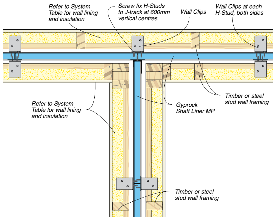
Figure 33: Junction Of Party Wall to Party Wall at T-Intersection (Option 2) – Plan View
