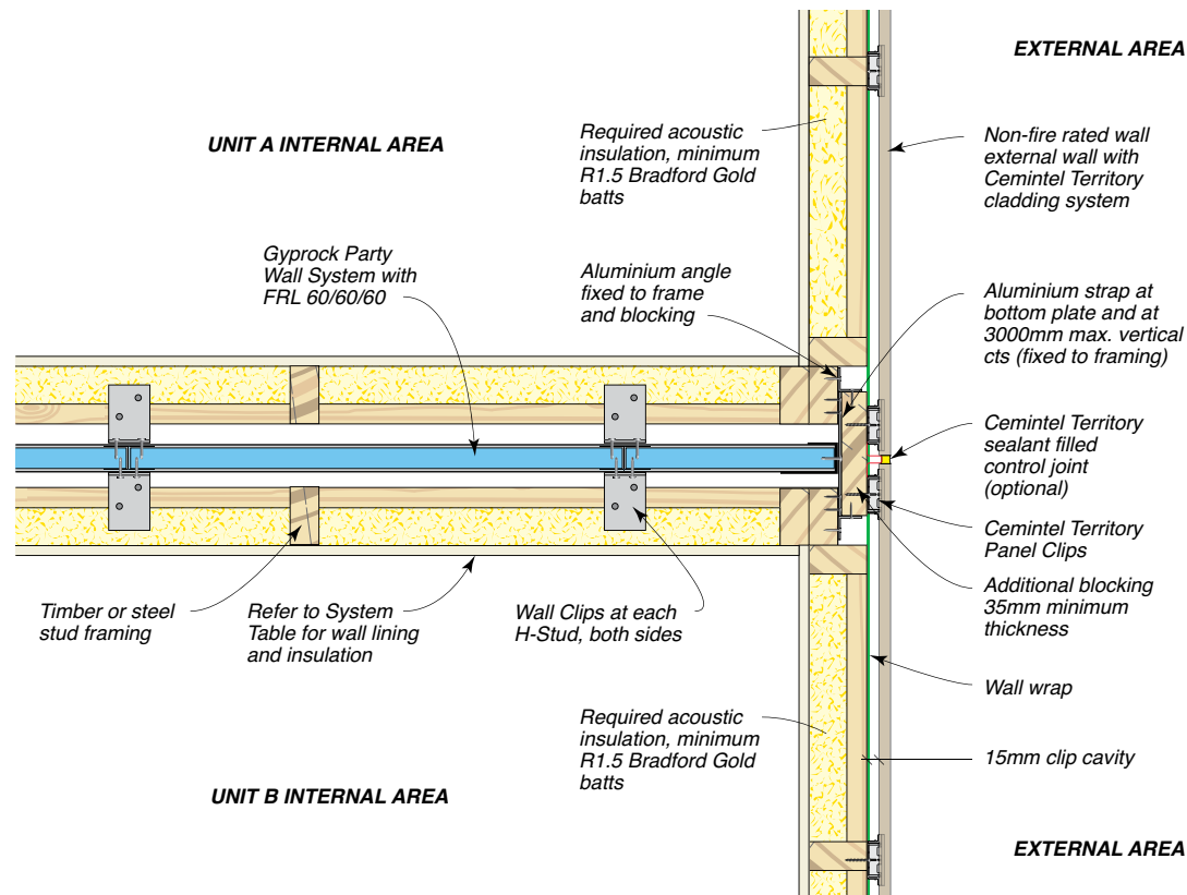
Figure 61: Junction Of Party Wall And External Wall With Cemintel Territory Series Cladding – Plan View
