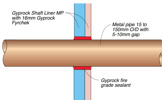
Figure 78: Metal Pipe Penetration – FRL –/90/–
