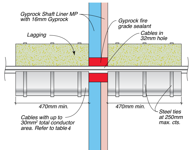
Figure 79: Insulated Electrical Cable Penetration – FRL –/90/60
