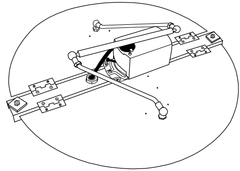
Type 5 Electric Butterfly Type Damper
